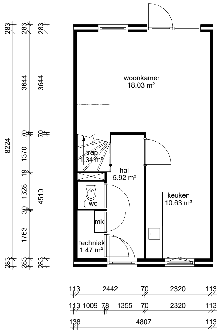
Begane_grond
