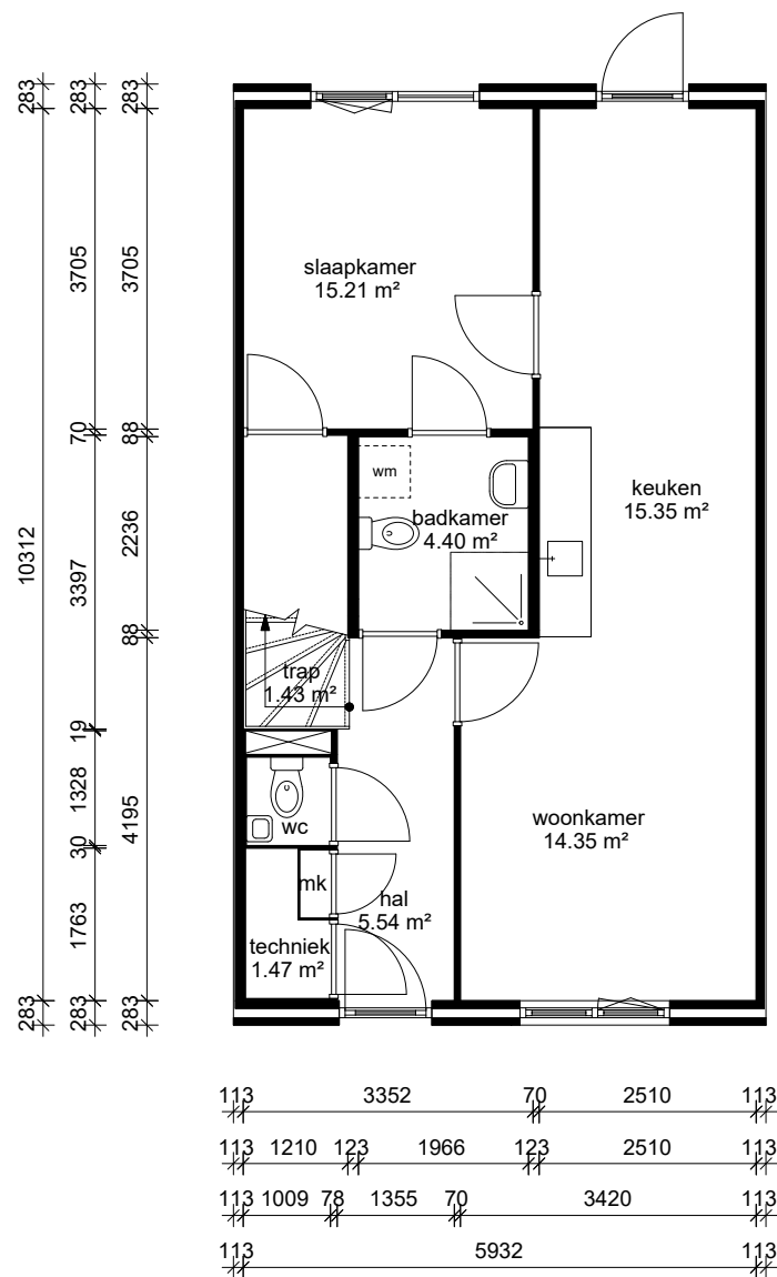
Begane_grond
